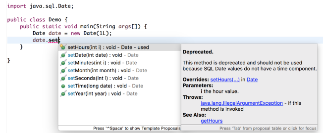
Figure 1: Example of deprecation warning in the IDE
